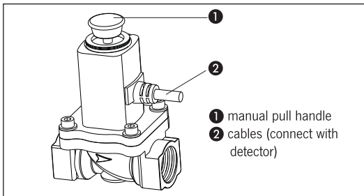
solenoid valve (optional accessory)
